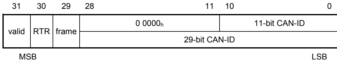
Figure 71: Structure of TPDO COB-ID
