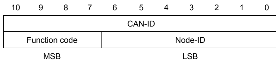
Figure 50: CAN-ID-allocation scheme for the generic pre-defined connection set
