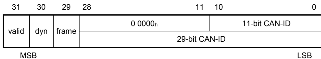
Figure 65: Structure of SDO server COB-ID
