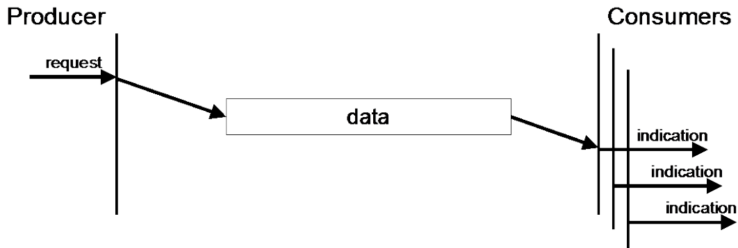
Figure 9: Push model
